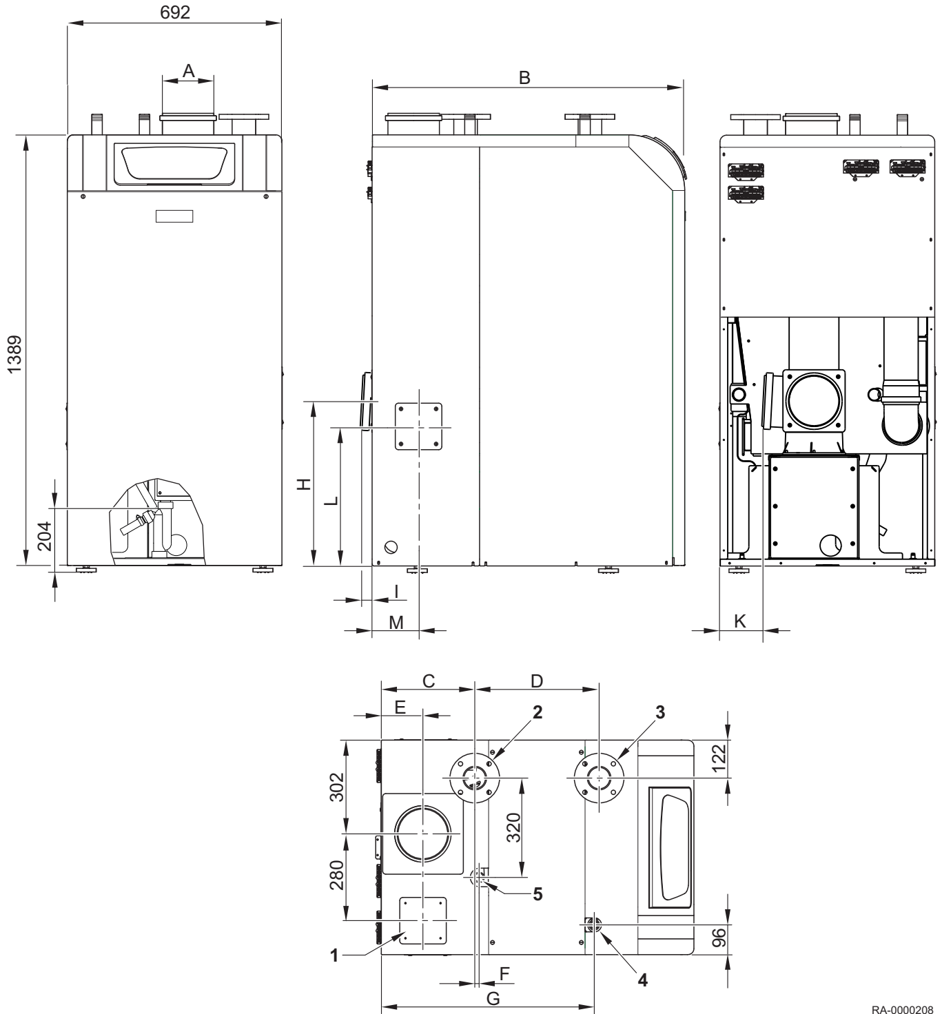
Fig.2 Dimensions et raccords
